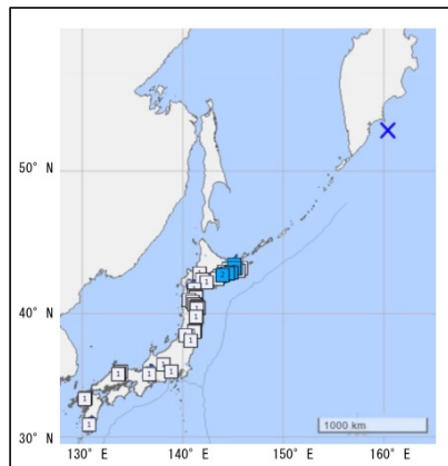
Observations of seismic intensity
