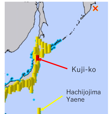
Maximum observed tsunami height in Japan
